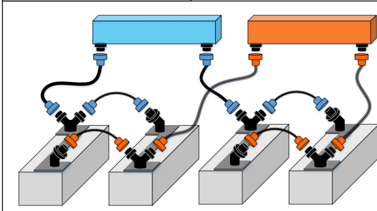
Detail A: Seed Delivery Installation
