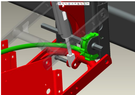
Illustration A: Cable Drive Contacts Delta Force Cylinder with Gear Box in Factory Installed Position
