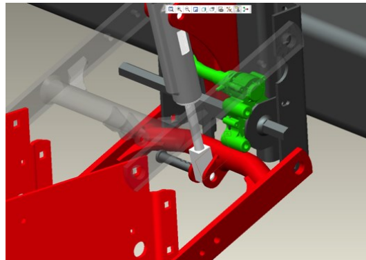
Illustration B: Cable Drive Contacts Delta Force Cylinder with Gear Box in Rotated to Upper Position
