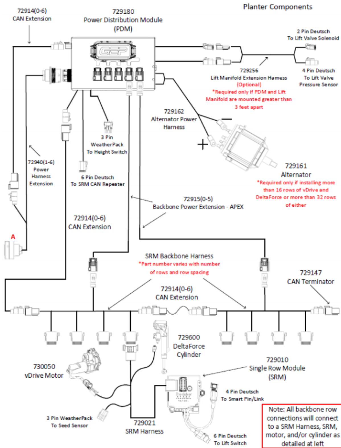
Figure 1. Harness Overview
