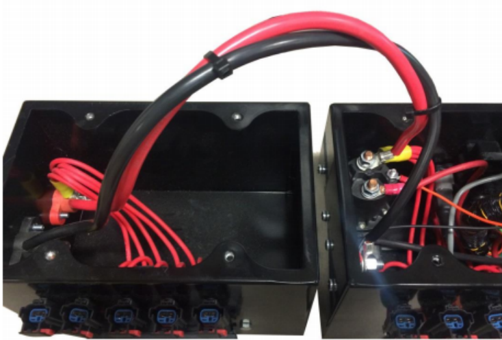
(Secondary PDM connected to Primary PDM)
