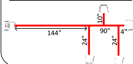
Dimensions of 725937 Sensor Backbone
