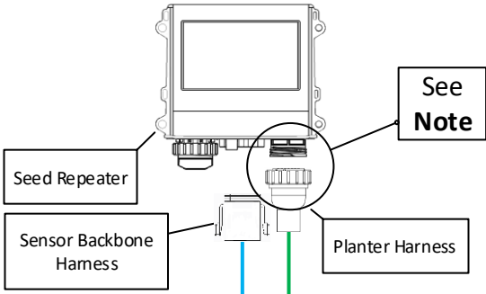
Detail A: Smart Connector Connections
