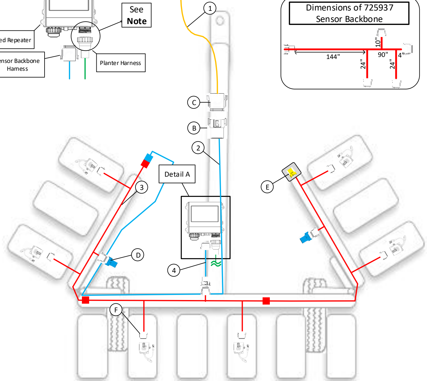
Detail A: Smart Connector Connections
