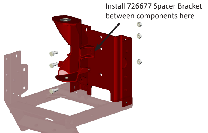
Case Air Spring Head Mount (726672) and 1/2" X 1.125" GRD5 Bolts (13206)
