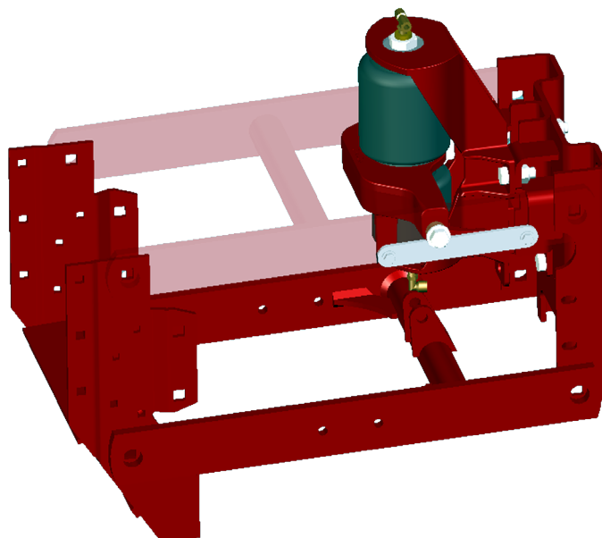
Complete Row Unit Conversion
