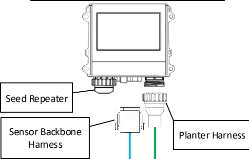
Detail A: Smart Connector Connections
